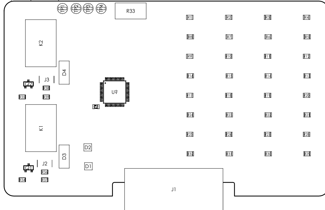
Front side (Scale 2:1)
